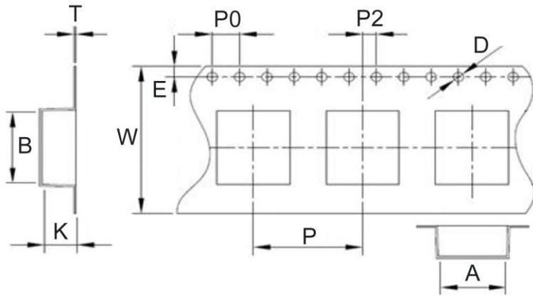
Tape Dimensions
