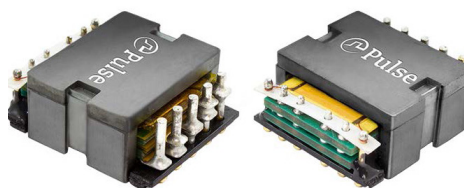
Electrical Specifications @ 25°C - Operating Temperature -40°C to +125°C
