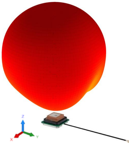
L1 3D RHCP Pattern @1575 MHz
