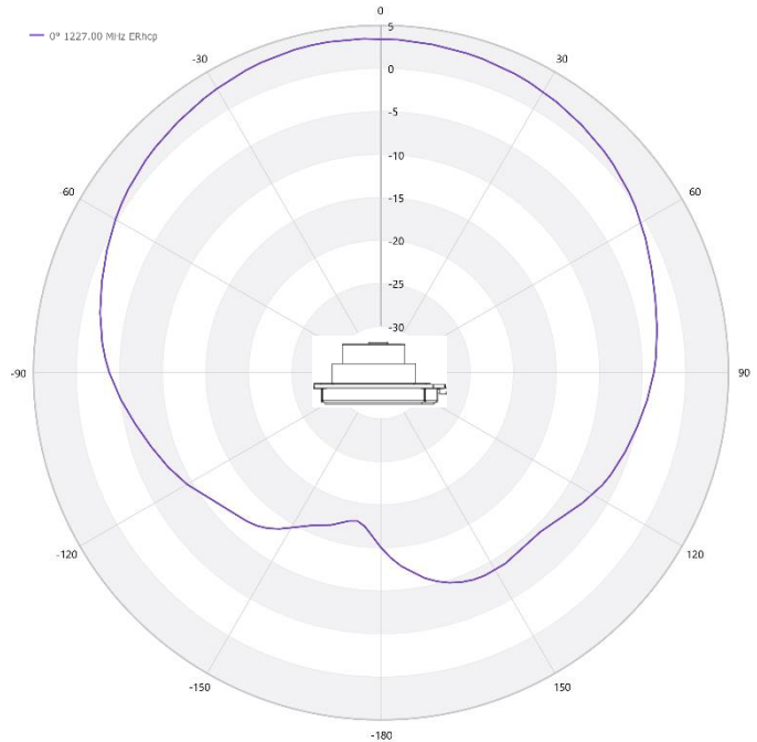
L2 RHCP Pattern
