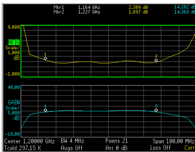
L2 Noise Figure
