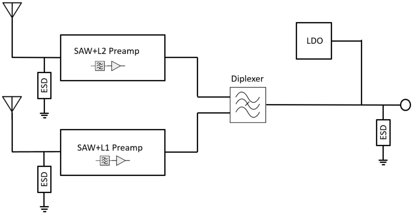
Active Antenna Block Diagram
