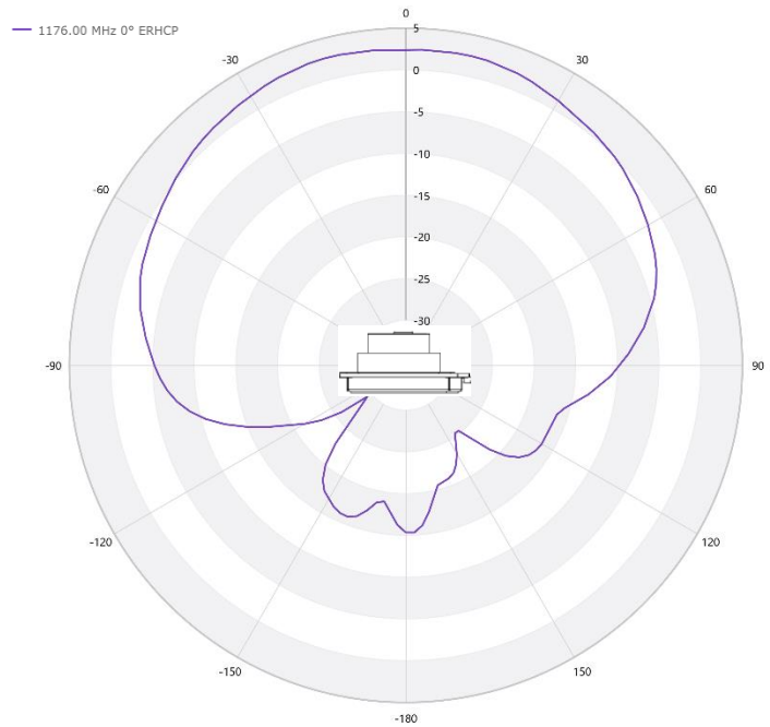
L5 RHCP Pattern
