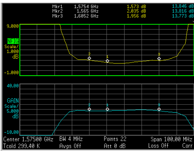
L1 Noise Figure
