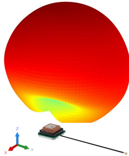
L5 3D RHCP Pattern @1176 MHz
