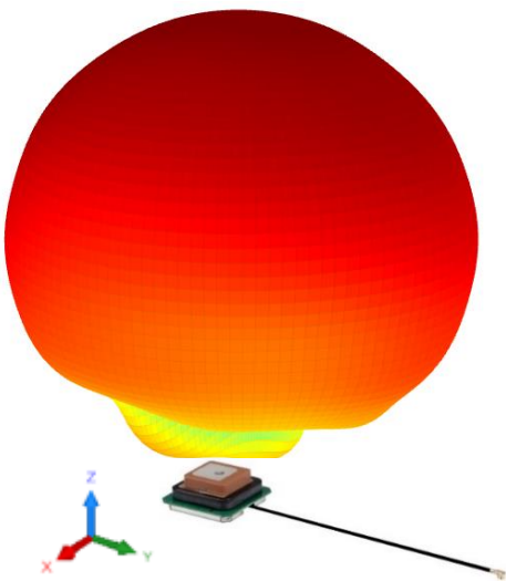
L1 3D RHCP Pattern @1575 MHz
