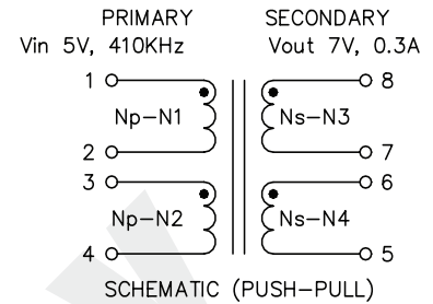
SCHEMATIC (PUSH-PULL)
