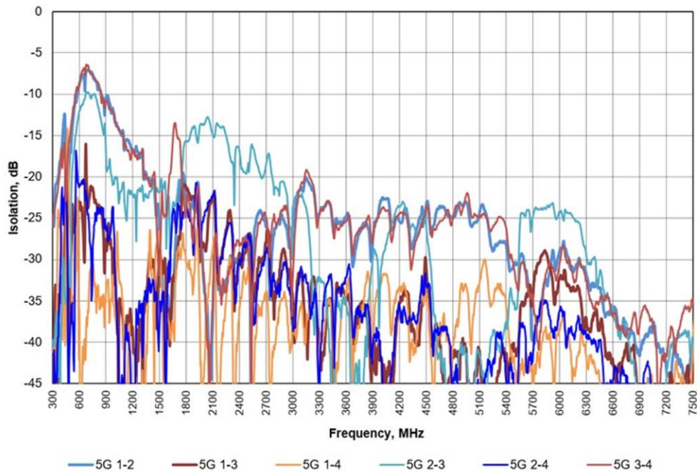
Isolation vs Frequency
