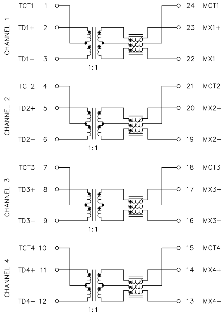
SCHEMATIC
